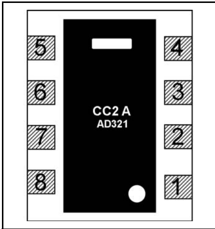
Figure 8: Pin Assignments
