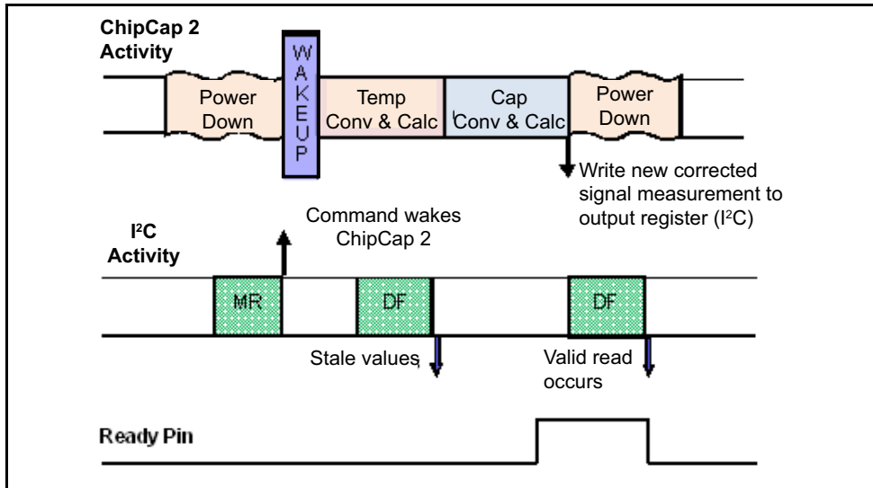
Figure 15: I 2 C Data Fetching in Sleep Mode
