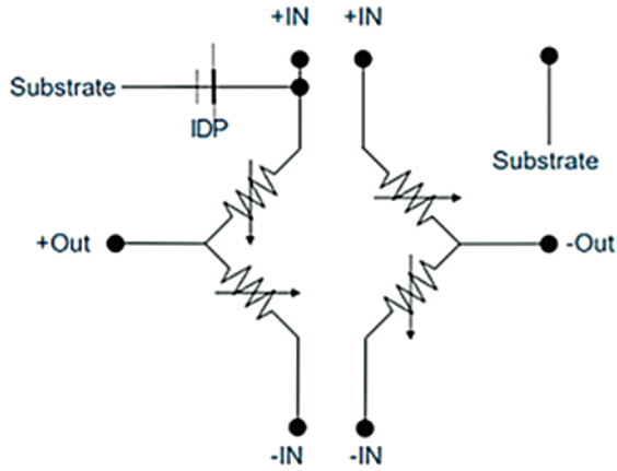
P1300 Schematic Diagram
