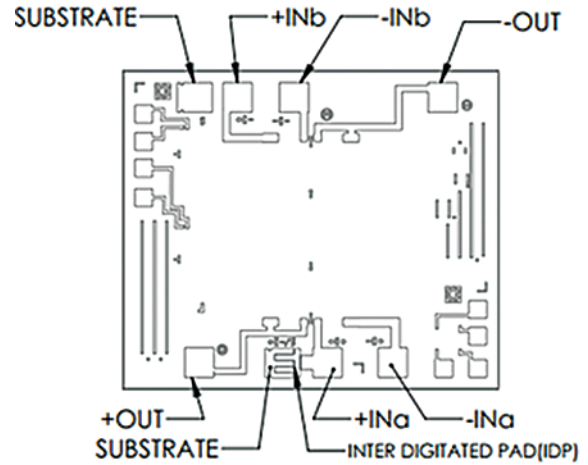
P1300 Wire Bond Diagram
